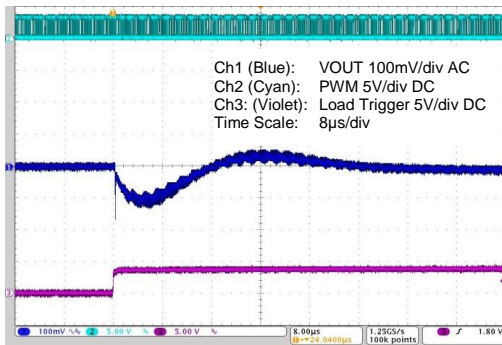
Figure 5.24 5 to 20A Load Step – Max. Capacitance
