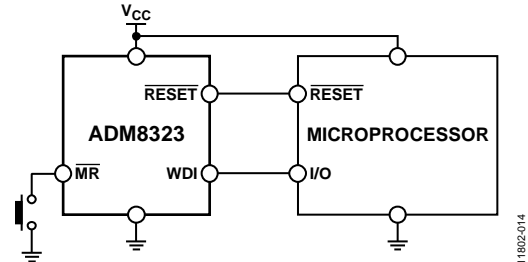
Figure 25. ADM8323 Typical Application Circuit
