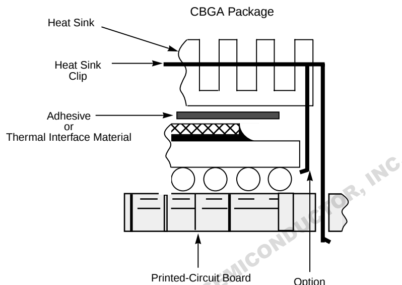
Figure 20. Package Exploded Cross-Sectional View with Several Heat Sink Options
