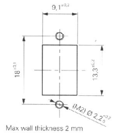
Max wall thickness 2 mm
