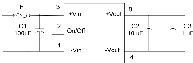
Figure 2. Typical Application of QTS48T46096
