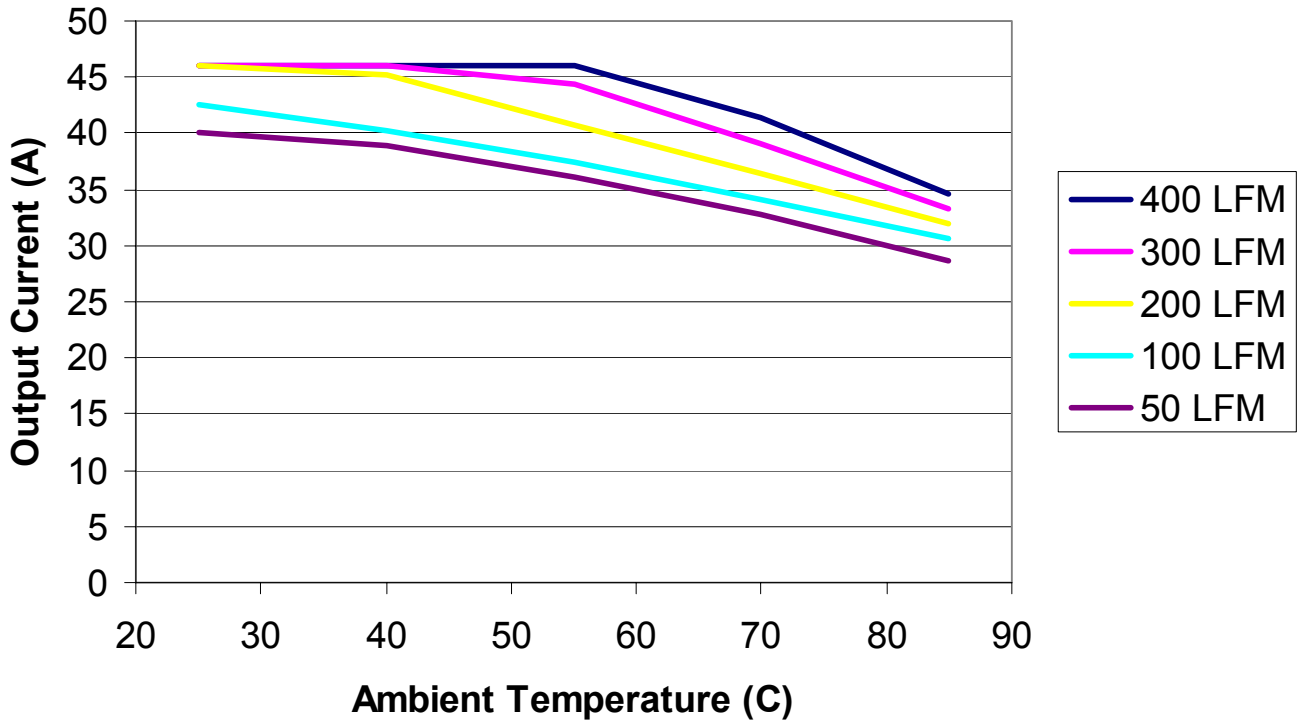
Figure 4. Thermal Derating Curve Vin = 36V, Varying Airflow (Input Voltage Constant)
