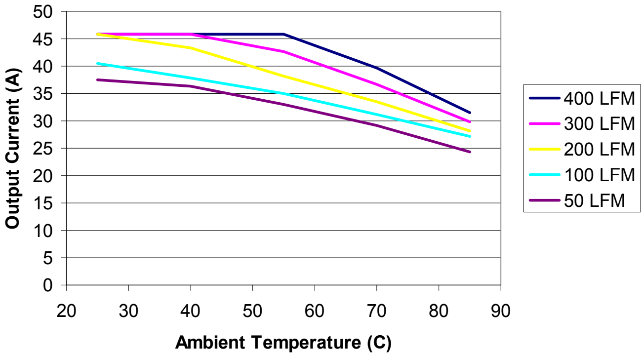
Figure 5. Thermal Derating Curve Vin = 48V, Varying Airflow (Input Voltage Constant)
