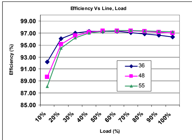
Figure 1. QTS48T46096 Efficiency vs. Output Load
