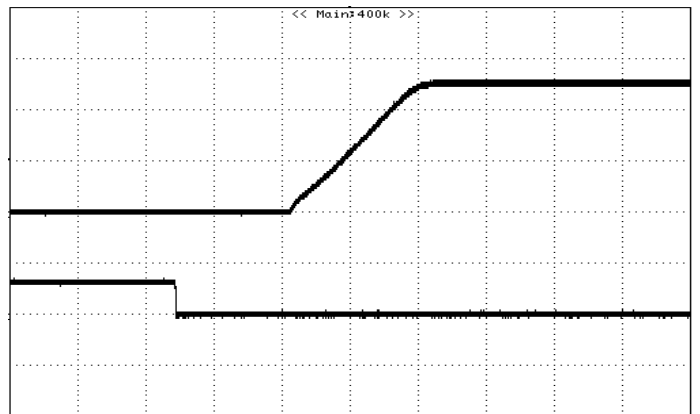
Figure 12: Turn on delay time at Remote On/Off, 5.0V/3A out (2mS/div). Top trace: Vout ,2V/div ;Bottom trace :ON/off , 5V/div.
