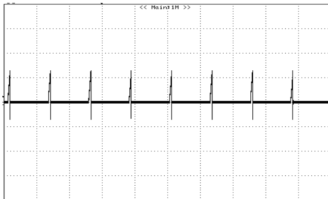
Figure 17: Output short circuit current 12Vin, 0.75Vout (0.5V/div,50mS/div)
