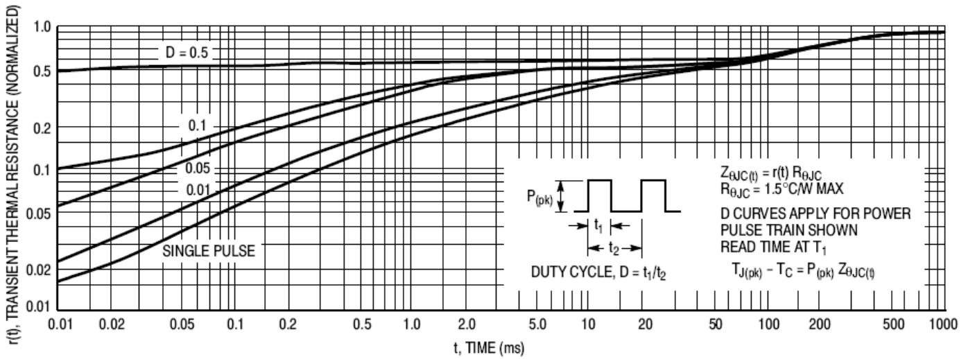
Figure 16. Thermal Response
