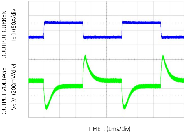
Figure 7. Transient response 12V DC output load step 10 – 60A, V IN = -48V DC .
