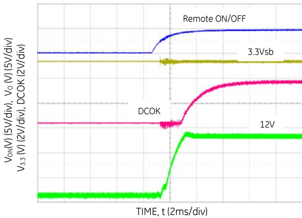
Figure 3. Start-up Using Remote On/Off ( V_{in} = -48V_{DC} , full load)
