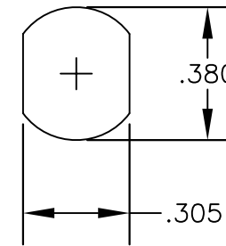
MOUNTING HOLE
