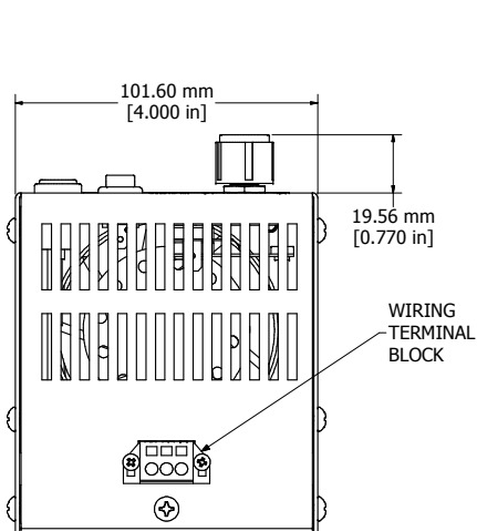
ASSEMBLY - VIEW FROM BOTTOM
