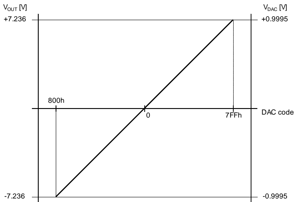
Figure 11. DAC Setting vs. V_{DAC}/V_{OUT} (in low gain mode)
