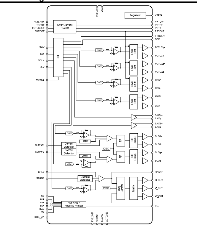
Figure 3. Block diagram
