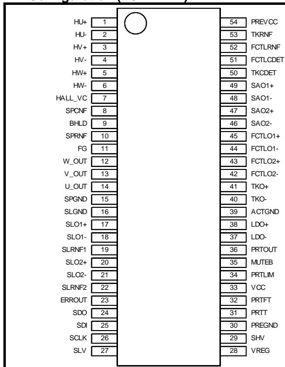
Figure 2. Pin configuration
