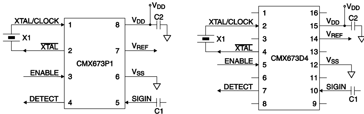
Figure 2: Recommended External Components
