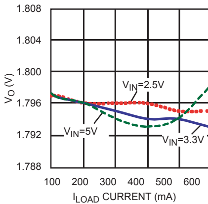
85 °C Load Regulation
