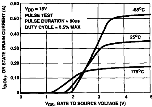
FIGURE 6. TRANSFER CHARACTERISTICS
