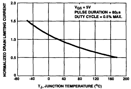
FIGURE 11. NORMALIZED DRAIN LIMITING CURRENT vs JUNCTION TEMPERATURE
