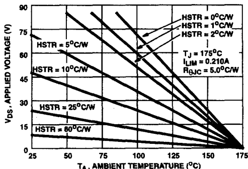
FIGURE 15. DC OPERATION IN CURRENT LIMITING
