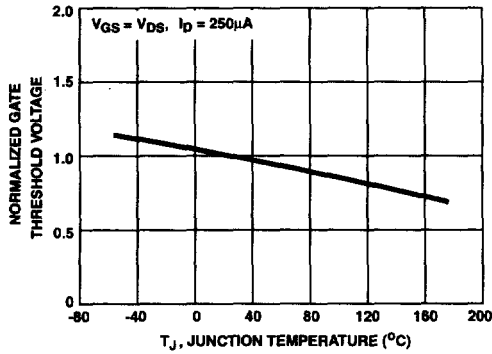
FIGURE 8. NORMALIZED GATE THRESHOLD VOLTAGE vs JUNCTION TEMPERATURE
