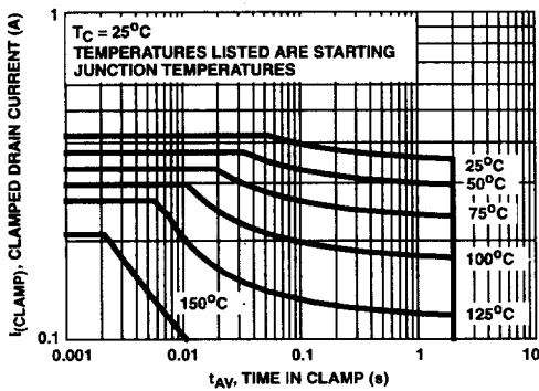
FIGURE 4. SELF-CLAMPED INDUCTIVE SWITCHING
