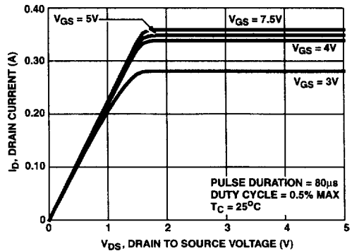
FIGURE 5. SATURATION CHARACTERISTICS
