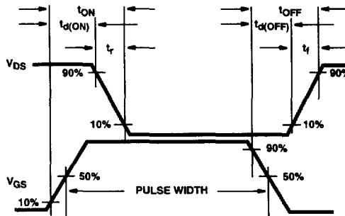
FIGURE 14. RESISTIVE SWITCHING WAVEFORMS
