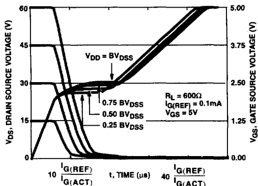
FIGURE 12. NORMALIZED SWITCHING WAVEFORMS FOR CONSTANT GATE CURRENT.
