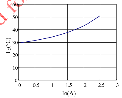
Case Temperature vs Output Current (Vin=5V, Vo=1.8V, Ta=27°C)
