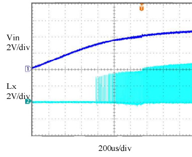
Soft Start(Lx)
