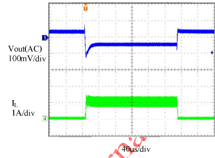
Load Transient (Vin=5.0V, Vout=1.8V, Iload=0-1A)
