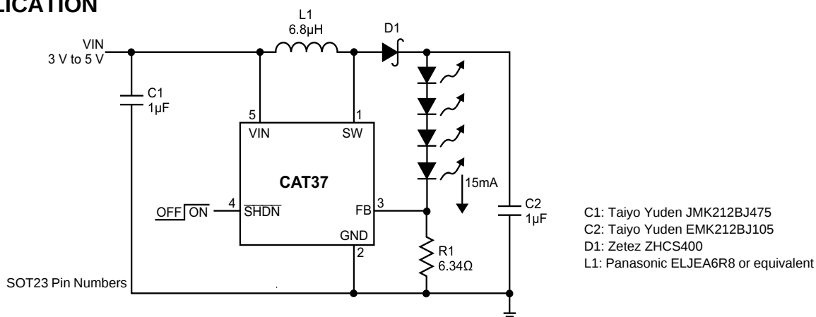
Figure 1. Driver for Four High-Brightness White LEDs
