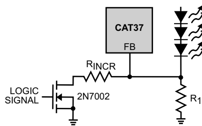
Figure 5. Dimming with a Logic Signal
