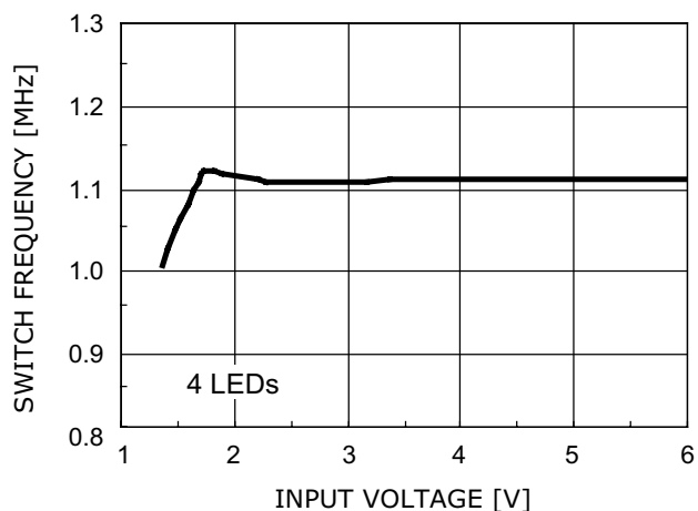
Switching Frequency vs. Input Voltage
