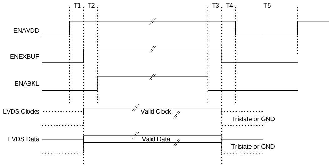
Figure 3: Power Sequencing
