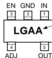
MIC5219BM5 SOT-23-5 Adjustable Voltage (Top View)
