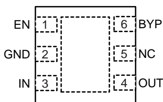
MIC5219-x.xBML 6-Pin 2mm x 2mm MLF™ (ML) (Top View)
