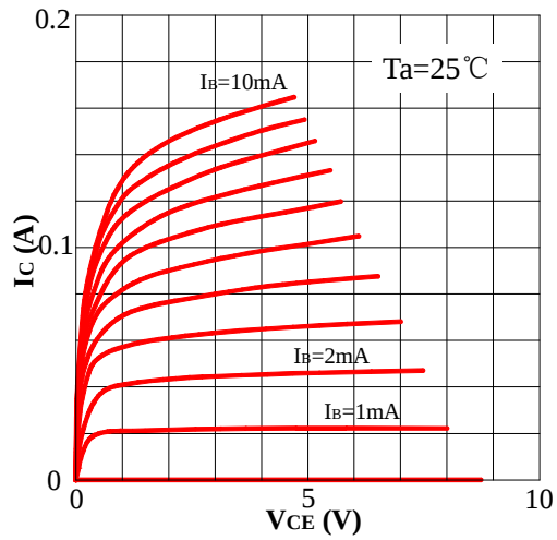
Fig1 Static Characteristic
