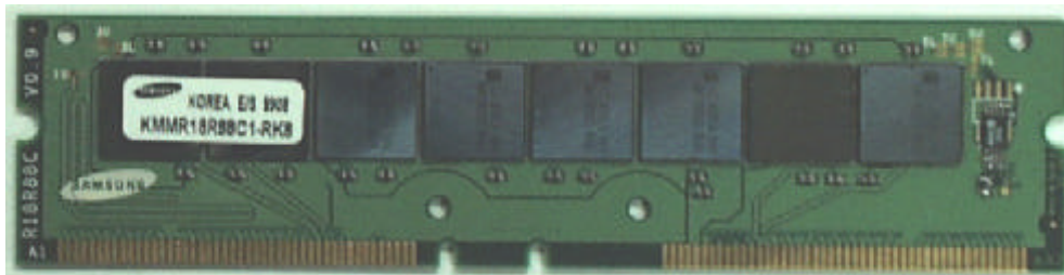
Note: On two sided modules, RDRAMs are also installed on bottom side of PCB.
