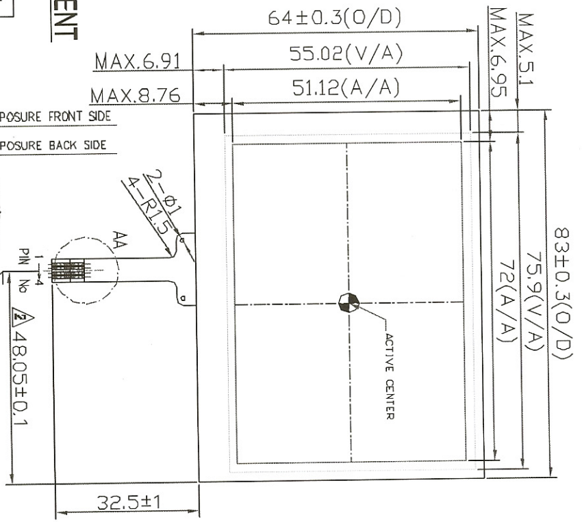
Detail "AA" (Scale=4/1)
