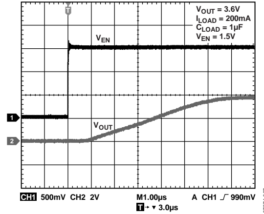
Figure 8. ADP190 Turn-On Delay, Input Voltage = 3.6\text{ V}
