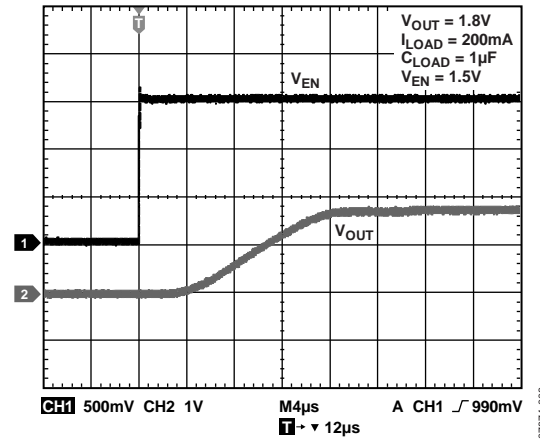
Figure 9. ADP190 Turn-On Delay, Input Voltage = 1.8\text{ V}
