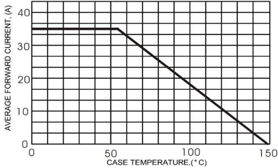
FIG.1 - TYPICAL FORWARD CORRENT DERATING CURVE
