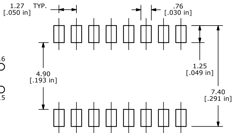
PC LAYOUT
