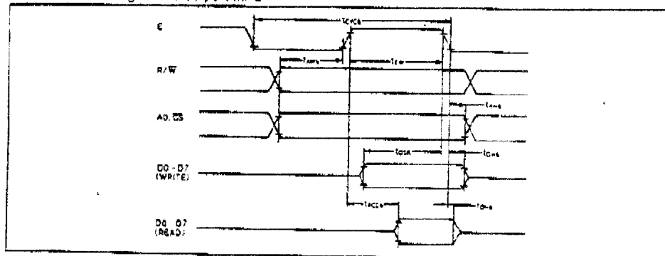
○ Control timing for 80-port/68-port display
