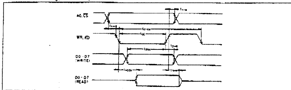
○ Read/Write timing for the 68-port MPU
