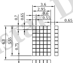
DOT SIZES SCALE 5/1
