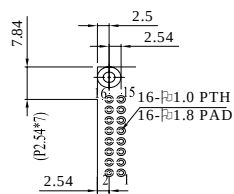
PIN DETAIL
