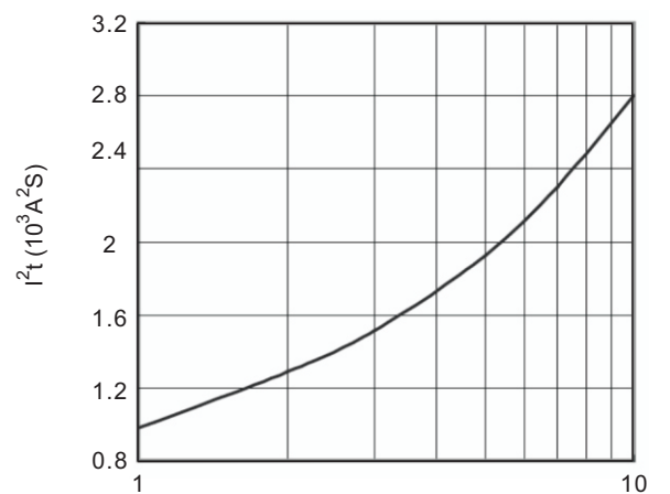
Fig.6 I 2 t characteristic
