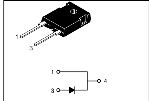
TO-247AD-2P Unit : inch (mm)
