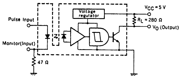
Test Circuit for Switching Time
