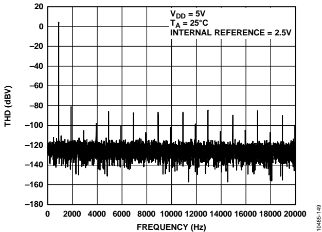
Figure 46. Total Harmonic Distortion @ 1 kHz
