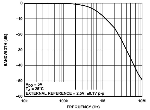
Figure 48. Multiplying Bandwidth, External Reference = 2.5 V, ±0.1 V p-p, 10 kHz to 10 MHz
