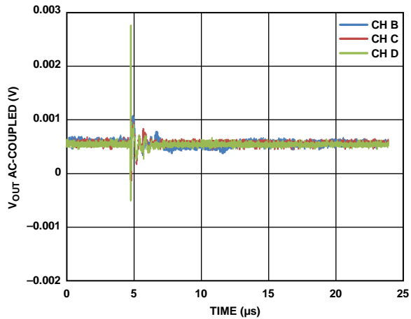
Figure 42. Analog Crosstalk, Channel A
