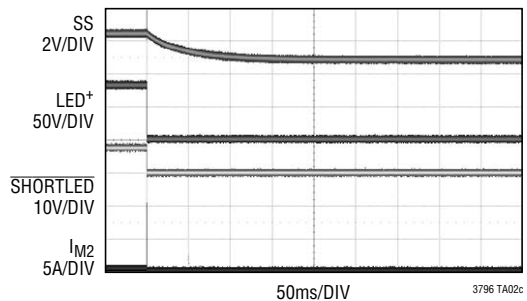
Short LED Protection with R11: Latchoff Mode
