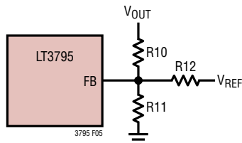
Figure 5. Feedback Resistor Connection for Wide Range Output in Boost and SEPIC Applications
