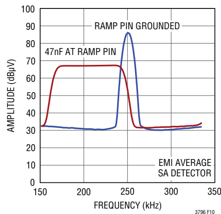
Figure 10. Input Noise Spectrum Comparison
