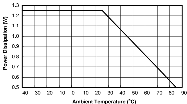
Figure 3. Derating Curves for APL3523A Package
