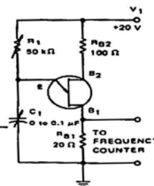
FIGURE 4 – f_{(max)} MAXIMUM FREQUENCY TEST CIRCUIT
