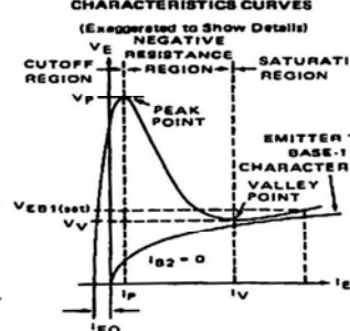
FIGURE 2 – STATIC EMITTER CHARACTERISTICS CURVES (Exaggerated to Show Details)
