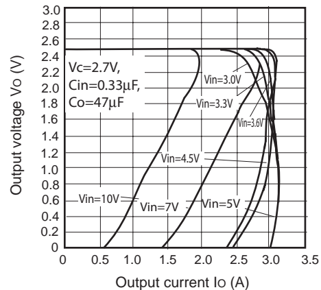
Fig.6 Overcurrent Protection Characteristics (PQ025EZ02ZxH)
