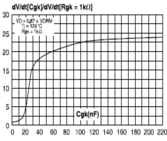
Fig.6 dv/dt VS C_{GK}
