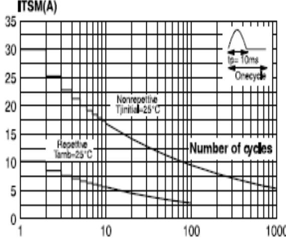
Fig. 4 I_{TSM} VS Number of cycles
