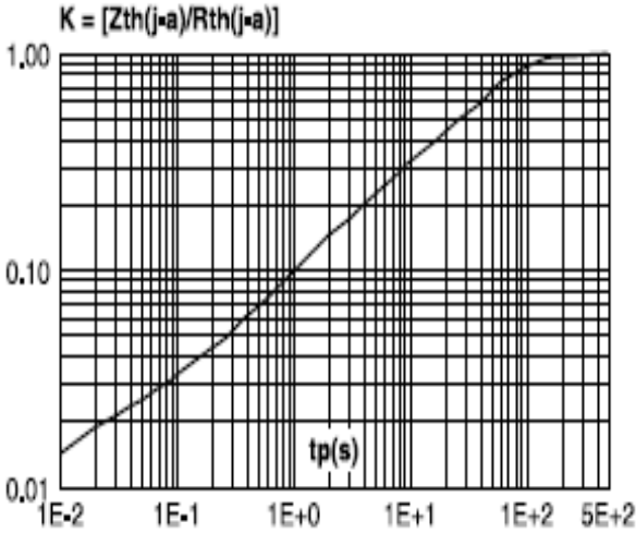
Fig.8 R_{\theta JA} VS Pulse duration
