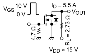
Fig. 6.2.1 Switching Time Test Circuit
