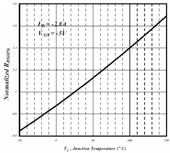
Fig 4. Normalized On-Resistance
