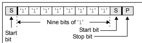
FIGURE 8-9: Software Reset Sequence Format.
