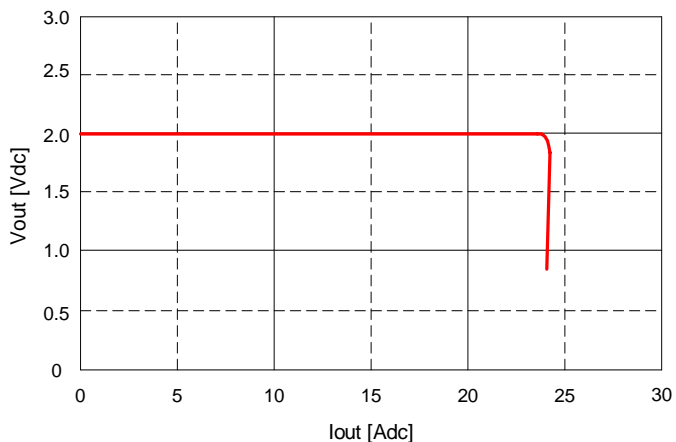
Fig. 2.0V.11: Output voltage vs. load current showing current limit point and converter shutdown point. Input voltage has almost no effect on current limit characteristic.
