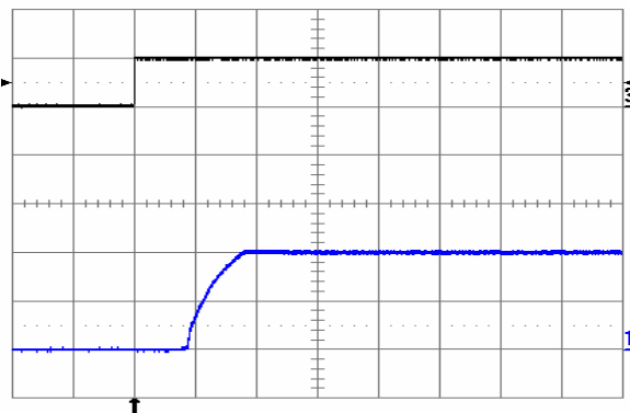
Fig. 2.0V.4: Turn-on transient at full rated load current (resistive) plus 10,000 \mu\text{F} at V_{in} = 48\text{ V} , triggered via ON/OFF pin. Top trace: ON/OFF signal (5 V/div.). Bottom trace: output voltage (1 V/div.). Time scale: 2 ms/div.
