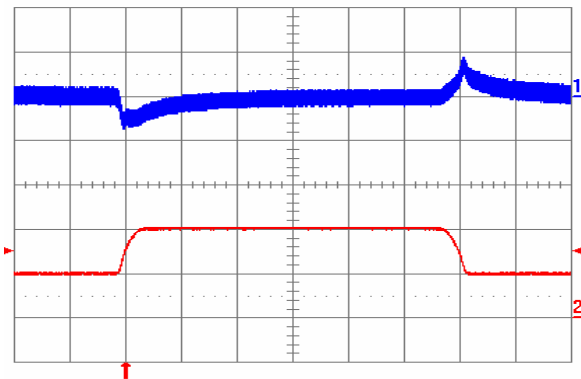
Fig. 3.3V.5: Output voltage response to load current step-change (5 A – 10 A – 5 A) at V_{in} = 48\text{ V} . Top trace: output voltage (100 mV/div.). Bottom trace: load current (5 A/div.). Current slew rate: 0.1 A/ \mu\text{s} . C_o = 1\ \mu\text{F} ceramic. Time scale: 0.2 ms/div.
