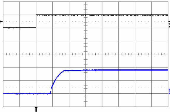
Fig. 1.8V.4: Turn-on transient at full rated load current (resistive) plus 10,000 \mu\text{F} at V_{in} = 48\text{ V} , triggered via ON/OFF pin. Top trace: ON/OFF signal (5 V/div.). Bottom trace: output voltage (1 V/div.). Time scale: 2 ms/div.
