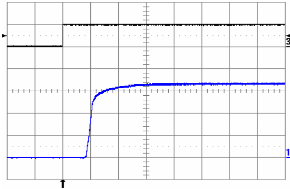
Fig. 3.3V.3: Turn-on transient at full rated load current (resistive) with no output capacitor at V_{in} = 48\text{ V} , triggered via ON/OFF pin. Top trace: ON/OFF signal (5 V/div.). Bottom trace: output voltage (1 V/div.). Time scale: 2 ms/div.
