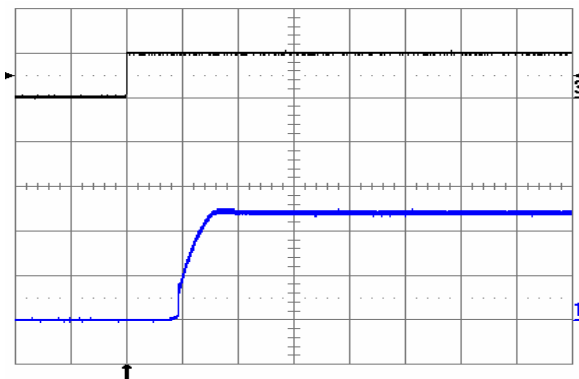
Fig. 1.2V.4: Turn-on transient at full rated load current (resistive) plus 10,000 \mu\text{F} at V_{in} = 48\text{ V} , triggered via ON/OFF pin. Top trace: ON/OFF signal (5 V/div.). Bottom trace: output voltage (0.5 V/div.). Time scale: 2 ms/div.
