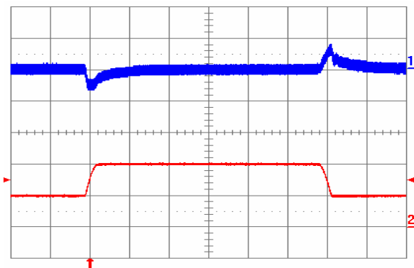
Fig. 2.0V.5: Output voltage response to load current step-change (5 A – 10 A – 5 A) at V_{in} = 48\text{ V} . Top trace: output voltage (100 mV/div.). Bottom trace: load current (5 A/div.). Current slew rate: 0.1 A/ \mu\text{s} . C_o = 1\ \mu\text{F} ceramic. Time scale: 0.2 ms/div.
