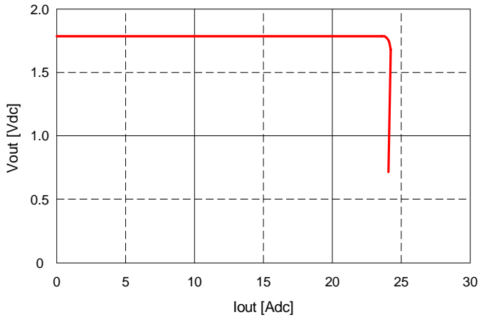
Fig. 1.8V.11: Output voltage vs. load current showing current limit point and converter shutdown point. Input voltage has almost no effect on current limit characteristic.
