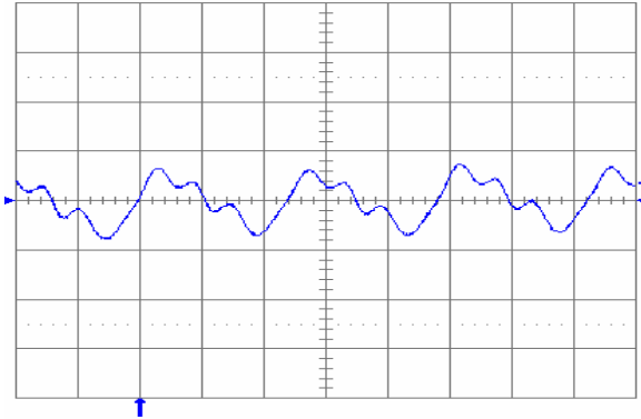
Fig. 3.3V.7: Output voltage ripple (20 mV/div.) at full rated load current into a resistive load with C_o = 10 \mu\text{F} tantalum + 1\mu\text{F} ceramic and V_{in} = 48 \text{ V} . Time scale: 1 \mu\text{s}/\text{div} .
