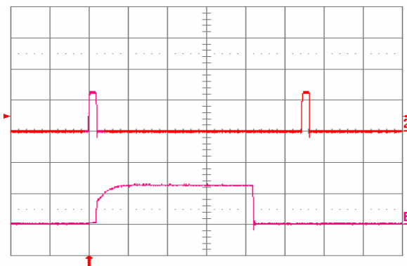
Fig. 1.5V.12: Load current (top trace, 20 A/div., 20 ms/div.) into a 10 mΩ short circuit during restart, at Vin = 48 V. Bottom trace (20 A/div., 1 ms/div.) is an expansion of the on-time portion of the top trace.
