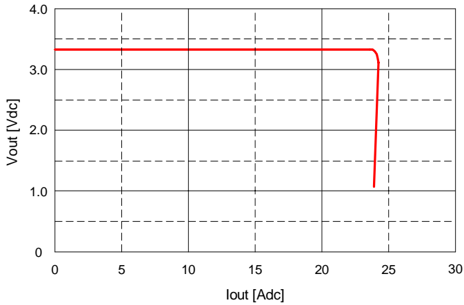
Fig. 3.3V.11: Output voltage vs. load current showing current limit point and converter shutdown point. Input voltage has almost no effect on current limit characteristic.
