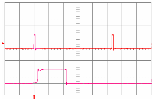
Fig. 2.5V.12: Load current (top trace, 20 A/div., 20 ms/div.) into a 10 mΩ short circuit during restart, at V in = 48 V. Bottom trace (20 A/div., 1 ms/div.) is an expansion of the on-time portion of the top trace.
