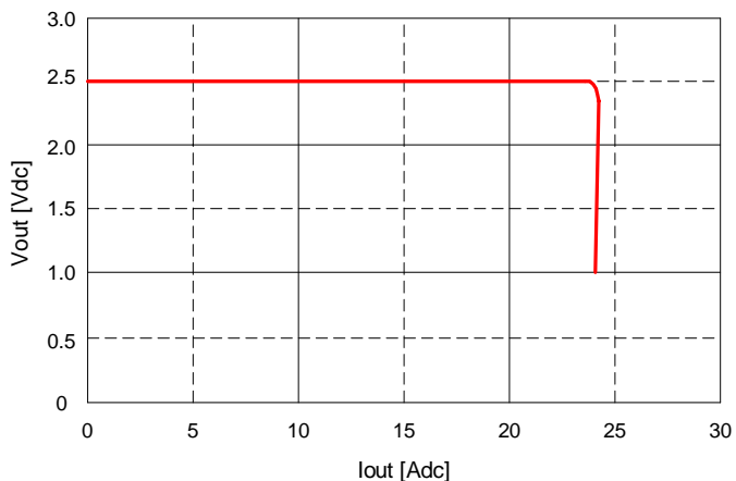
Fig. 2.5V.11: Output voltage vs. load current showing current limit point and converter shutdown point. Input voltage has almost no effect on current limit characteristic.
