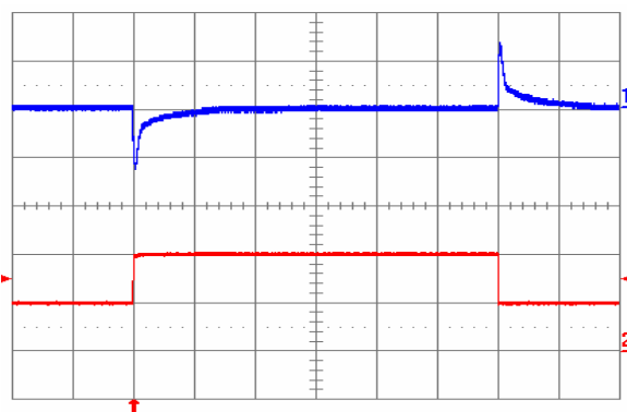
Fig. 2.0V.6: Output voltage response to load current step-change (5 A – 10 A – 5 A) at V_{in} = 48\text{ V} . Top trace: output voltage (100 mV/div.). Bottom trace: load current (5 A/div.). Current slew rate: 5 A/ \mu\text{s} . C_o = 450\ \mu\text{F} tantalum + 1 \mu\text{F} ceramic. Time scale: 0.2 ms/div.
