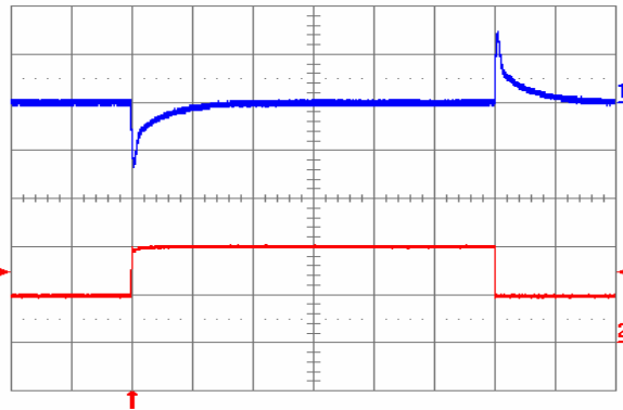
Fig. 1.8V.6: Output voltage response to load current step-change (5 A – 10 A – 5 A) at V_{in} = 48\text{ V} . Top trace: output voltage (100 mV/div.). Bottom trace: load current (5 A/div.). Current slew rate: 5 A/ \mu\text{s} . C_o = 450\ \mu\text{F} tantalum + 1 \mu\text{F} ceramic. Time scale: 0.2 ms/div.
