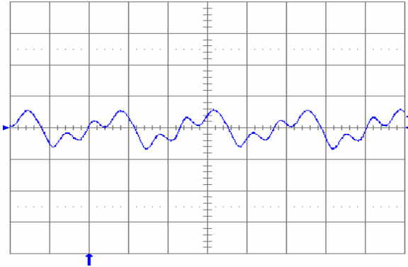
Fig. 2.0V.7: Output voltage ripple (20 mV/div.) at full rated load current into a resistive load with C_o = 10 \mu\text{F} tantalum + 1 \mu\text{F} ceramic and V_{in} = 48 \text{ V} . Time scale: 1 \mu\text{s}/\text{div} .
