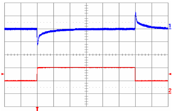
Fig. 3.3V.6: Output voltage response to load current step-change (5 A – 10 A – 5 A) at V_{in} = 48\text{ V} . Top trace: output voltage (100 mV/div.). Bottom trace: load current (5 A/div.). Current slew rate: 5 A/ \mu\text{s} . C_o = 450\ \mu\text{F} tantalum + 1 \mu\text{F} ceramic. Time scale: 0.2 ms/div.
