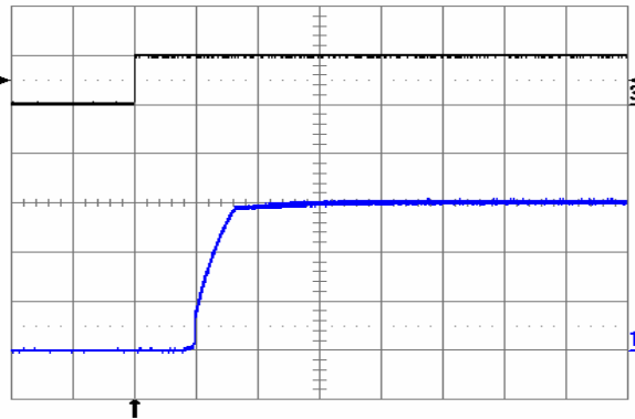
Fig. 1.5V.4: Turn-on transient at full rated load current (resistive) plus 10,000 \mu\text{F} at V_{in} = 48\text{ V} , triggered via ON/OFF pin. Top trace: ON/OFF signal (5 V/div.). Bottom trace: output voltage (0.5 V/div.). Time scale: 2 ms/div.
