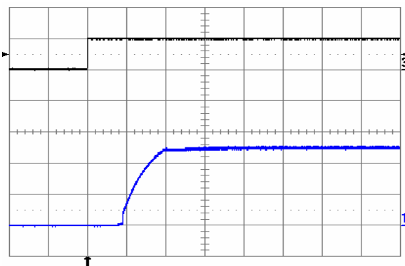
Fig. 2.5V.4: Turn-on transient at full rated load current (resistive) plus 10,000 \mu\text{F} at V_{in} = 48\text{ V} , triggered via ON/OFF pin. Top trace: ON/OFF signal (5 V/div.). Bottom trace: output voltage (1 V/div.). Time scale: 2 ms/div.
