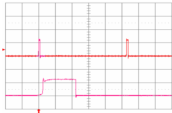
Fig. 2.0V.12: Load current (top trace, 20 A/div., 20 ms/div.) into a 10 mΩ short circuit during restart, at V in = 48 V. Bottom trace (20 A/div., 1 ms/div.) is an expansion of the on-time portion of the top trace.
