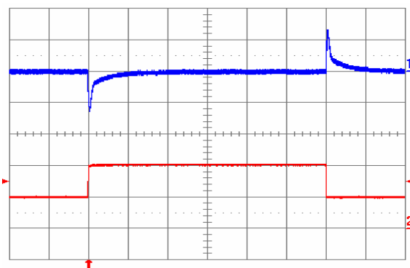
Fig. 2.5V.6: Output voltage response to load current step-change (5 A – 10 A – 5 A) at V_{in} = 48\text{ V} . Top trace: output voltage (100 mV/div.). Bottom trace: load current (5 A/div.). Current slew rate: 5 A/ \mu\text{s} . C_o = 450\ \mu\text{F} tantalum + 1 \mu\text{F} ceramic. Time scale: 0.2 ms/div.
