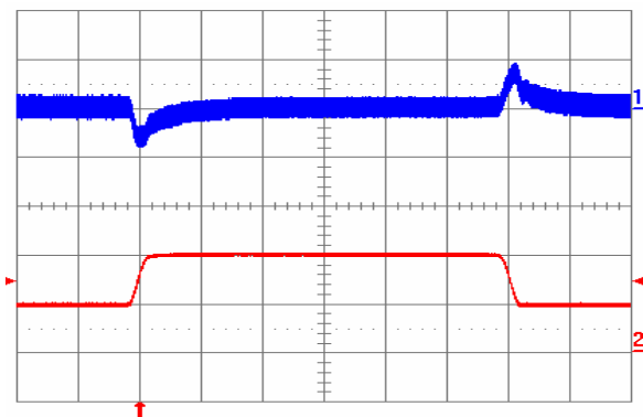
Fig. 1.2V.5: Output voltage response to load current step-change (5 A – 10 A – 5 A) at V_{in} = 48\text{ V} . Top trace: output voltage (100 mV/div.). Bottom trace: load current (5 A/div.). Current slew rate: 0.1 A/ \mu\text{s} . C_o = 1\ \mu\text{F} ceramic. Time scale: 0.2 ms/div.
