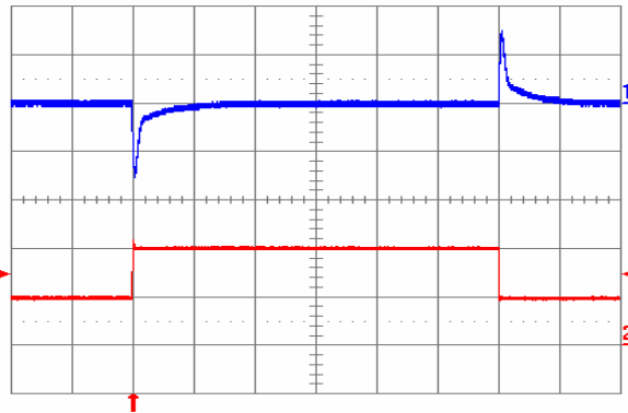
Fig. 1.5V.6: Output voltage response to load current step-change (5 A – 10 A – 5 A) at V_{in} = 48\text{ V} . Top trace: output voltage (100 mV/div.). Bottom trace: load current (5 A/div.). Current slew rate: 5 A/ \mu\text{s} . C_o = 450\ \mu\text{F} tantalum + 1 \mu\text{F} ceramic. Time scale: 0.2 ms/div.
