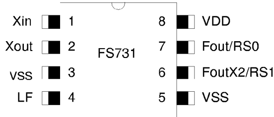
Figure 2. FS731, SOIC Package Pin Assignment
