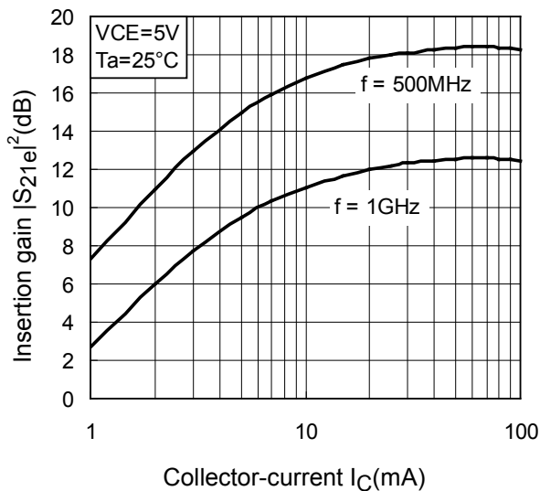
|S_{21e}|^2-I_C
