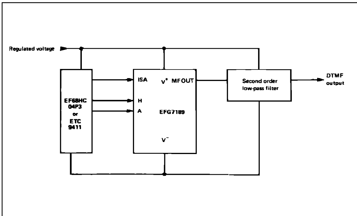
Figure 9 : Serial Connection.
