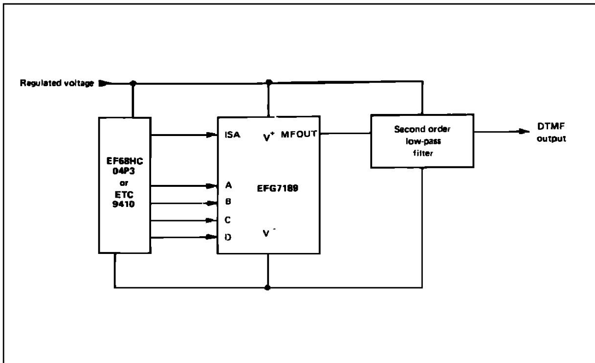
Figure 8 : Parallel Connection.
