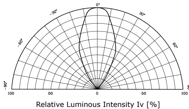
Fig. 5 Radiation Diagram
