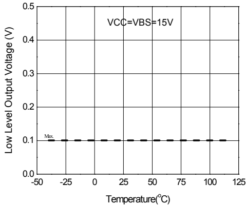
Figure 18a. Low Level Output of HO vs Temperature
