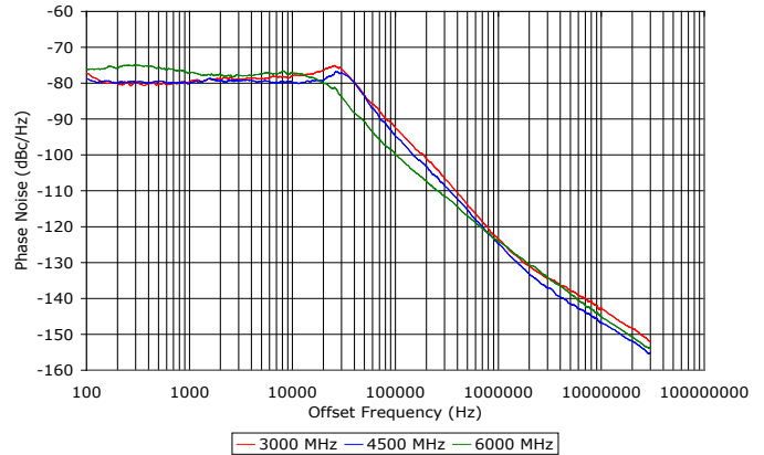
Phase Noise
