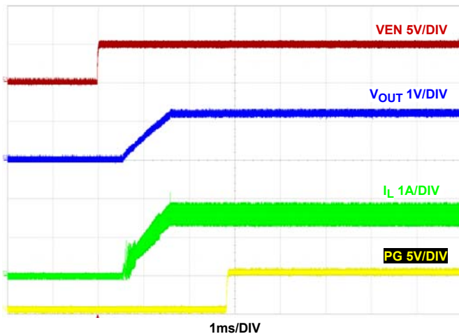
FIGURE 31. START-UP AT 1.5A LOAD F_{SW} = 2\text{MHz} , V_{IN} = 5\text{V} , \text{MODE} = \text{PFM} , T_A = +25^\circ\text{C}
