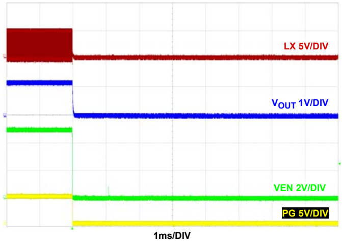
FIGURE 28. SHUTDOWN AT 2A LOAD F_{SW} = 2\text{MHz} , V_{IN} = 5\text{V} , \text{MODE} = \text{PFM} , T_A = +25^\circ\text{C}
