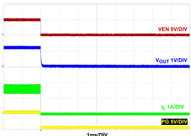
FIGURE 32. SHUTDOWN AT 1.5A LOAD F_{SW} = 2\text{MHz} , V_{IN} = 5\text{V} , \text{MODE} = \text{PFM} , T_A = +25^\circ\text{C}
