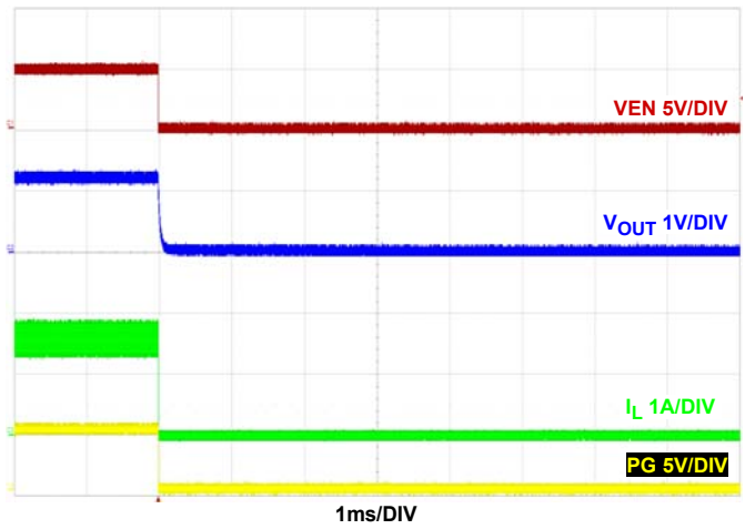
FIGURE 30. SHUTDOWN AT 1.5A LOAD F_{SW} = 2\text{MHz} , V_{IN} = 5\text{V} , \text{MODE} = \text{PWM} , T_A = +25^\circ\text{C}
