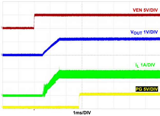
FIGURE 29. START-UP AT 1.5A LOAD F_{SW} = 2\text{MHz} , V_{IN} = 5\text{V} , \text{MODE} = \text{PWM} , T_A = +25^\circ\text{C}
