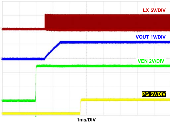
FIGURE 27. START-UP AT 2A LOAD F_{SW} = 2\text{MHz} , V_{IN} = 5\text{V} , \text{MODE} = \text{PFM} , T_A = +25^\circ\text{C}
