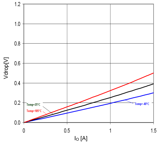
Figure 36. Minimum dropout Voltage 2 (V CC =8V, Ta=25°C)
