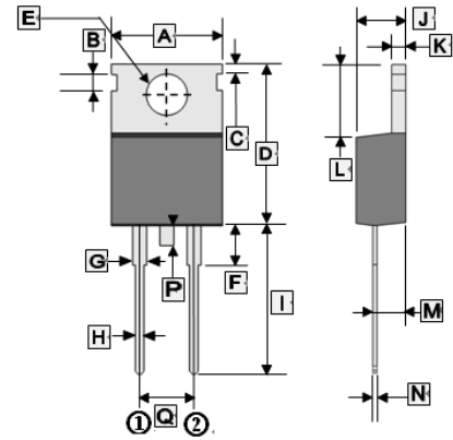
TO-220YA
