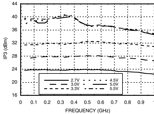
IP3 vs. Supply Voltage
