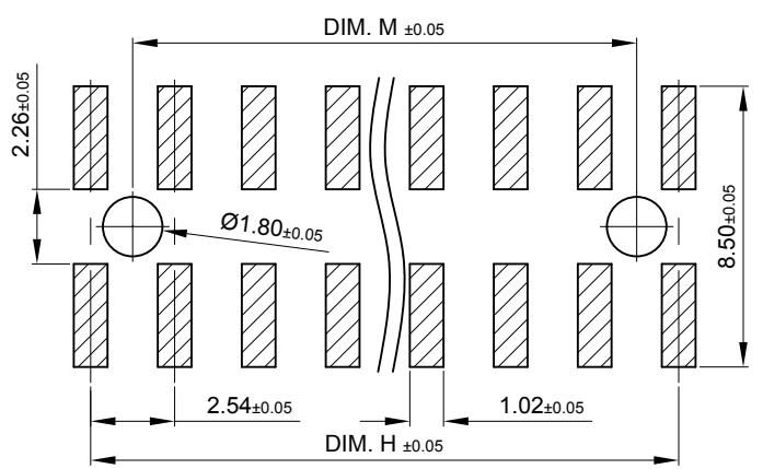
PCB Layout
